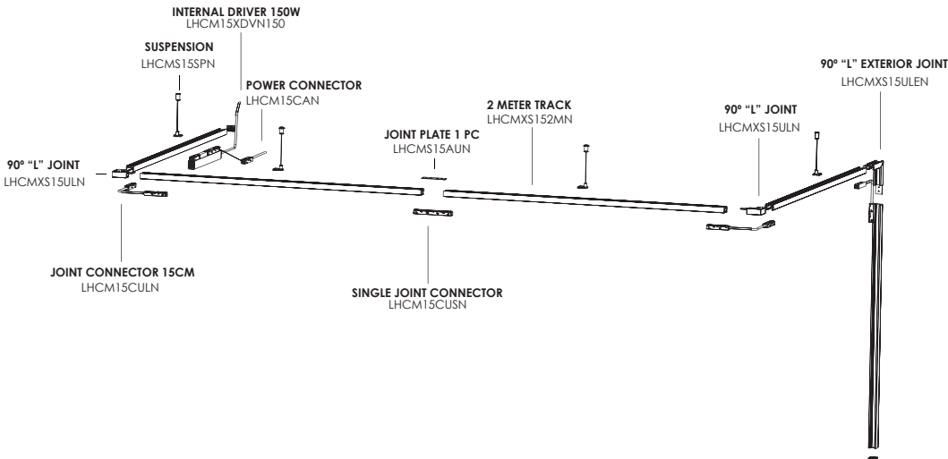
INTERNAL DRIVER 150W DC48V (225 x 41 x 21mm) LHCM15XDVN150 Black LHCM15XDVB150 White
