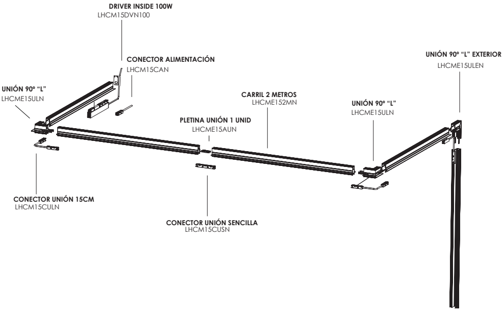
DRIVER INSIDE 100W DC48V / 200W LHCM15DVN100 (225 x 41 x 21mm) LHCM15DVN200 (305 x 43 x 21mm)
